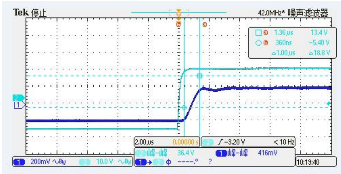
Fig.2 the step response time of STB-HA/Y current sensors. The light blue is primary current, while the dark blue is output signal of current sensor. The step response time is less than 1.5 μs.
