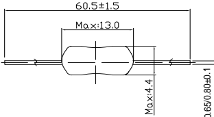
Dimensions (units: mm)
