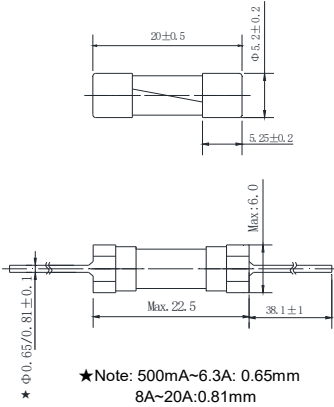
Dimensions (unit: mm)
