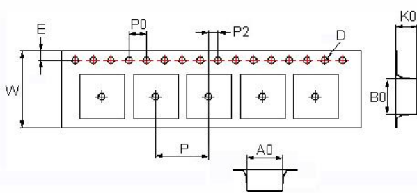
Tape Dimensions
