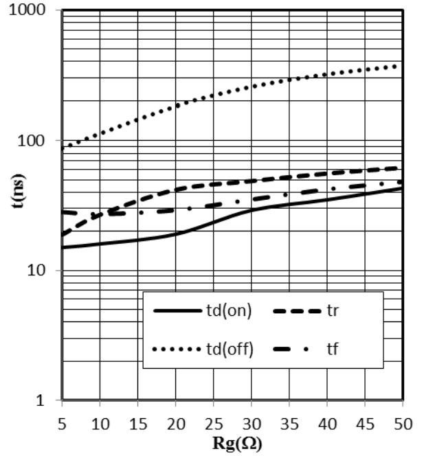
Fig 14. Typical switch time as a function of R_g (inductive load, T_j=25^\circ\text{C} , V_{CE}=400\text{V} , V_{GE}=15\text{V} , I_c=20\text{A} )
